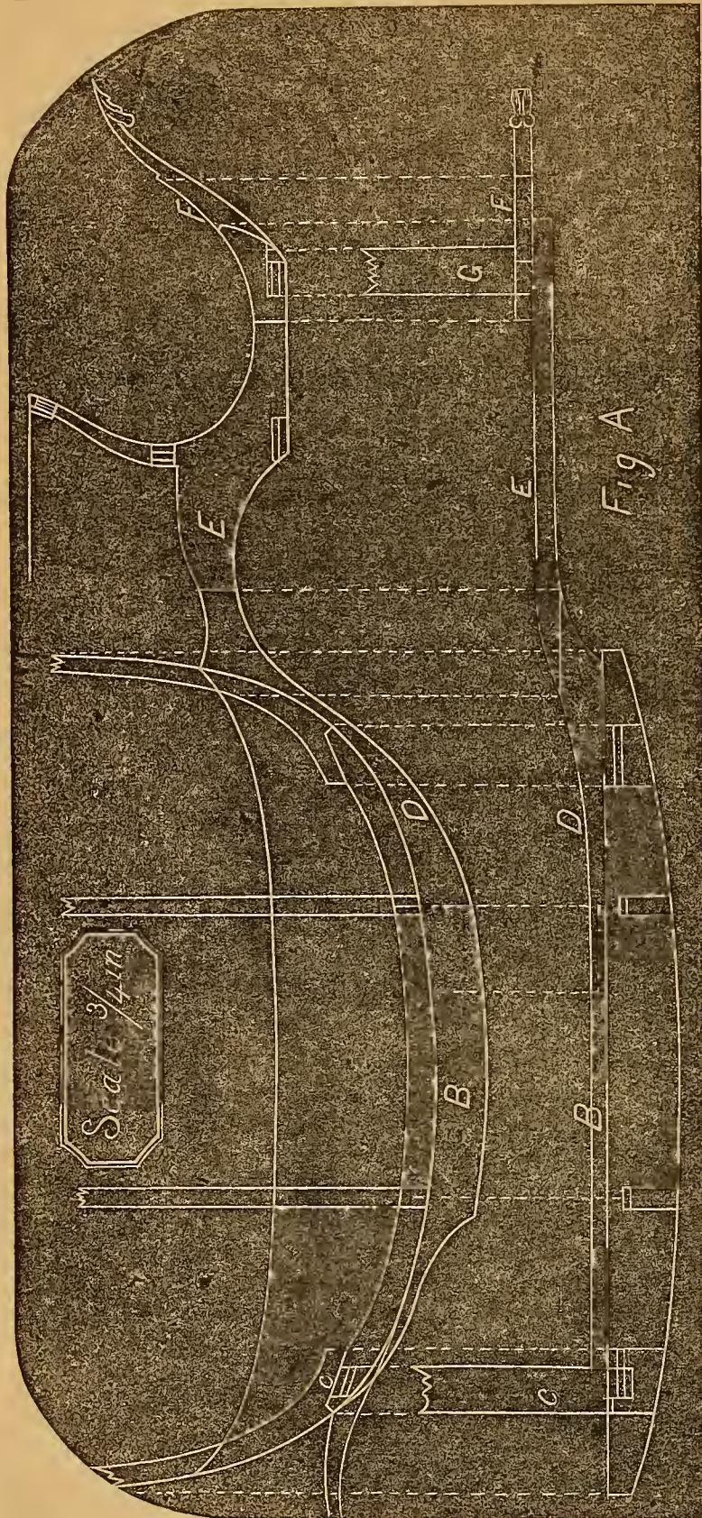
ROCKER WORK OF COACH, ON PLATE 43, VOL. I.
